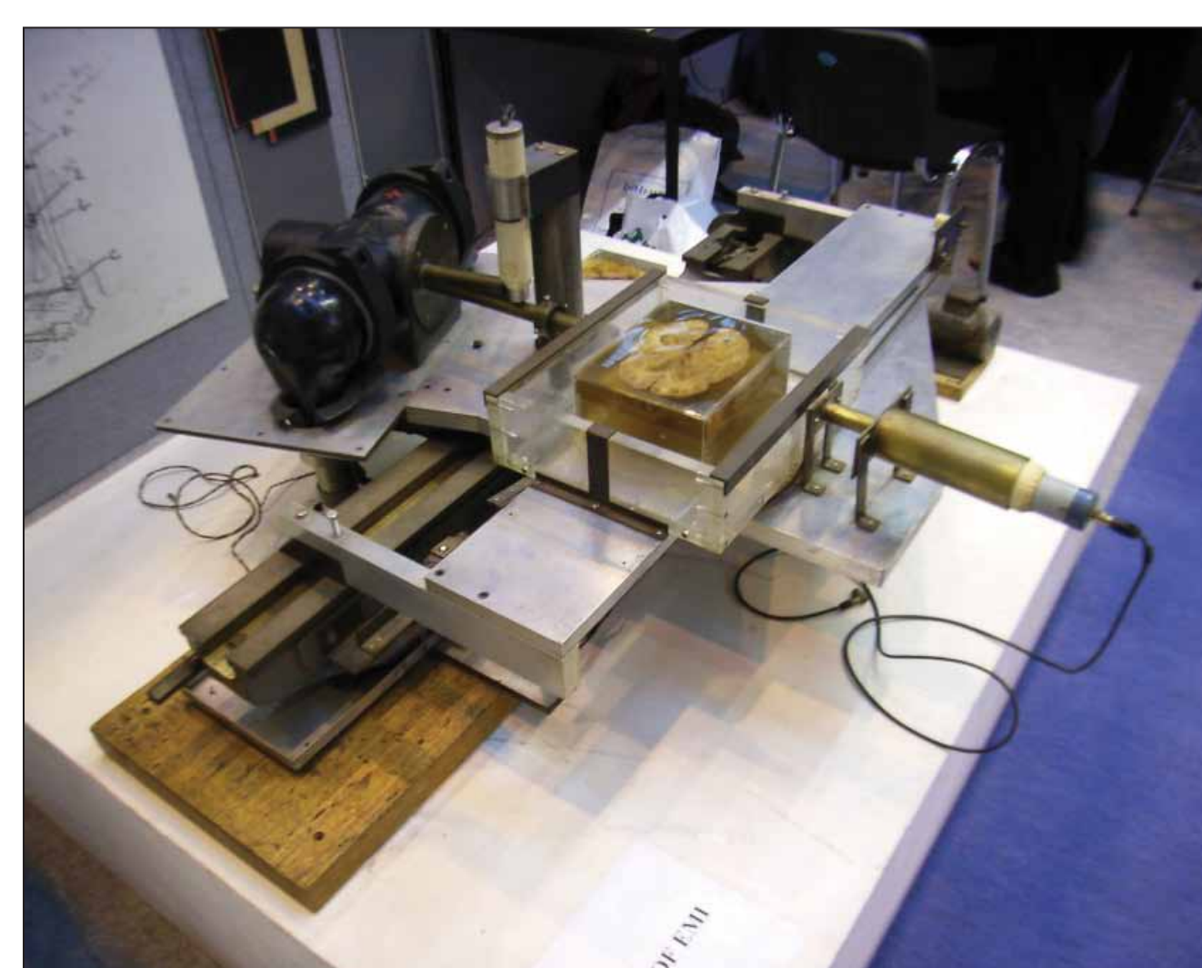
Figure 2. The experimental CT scanner.
