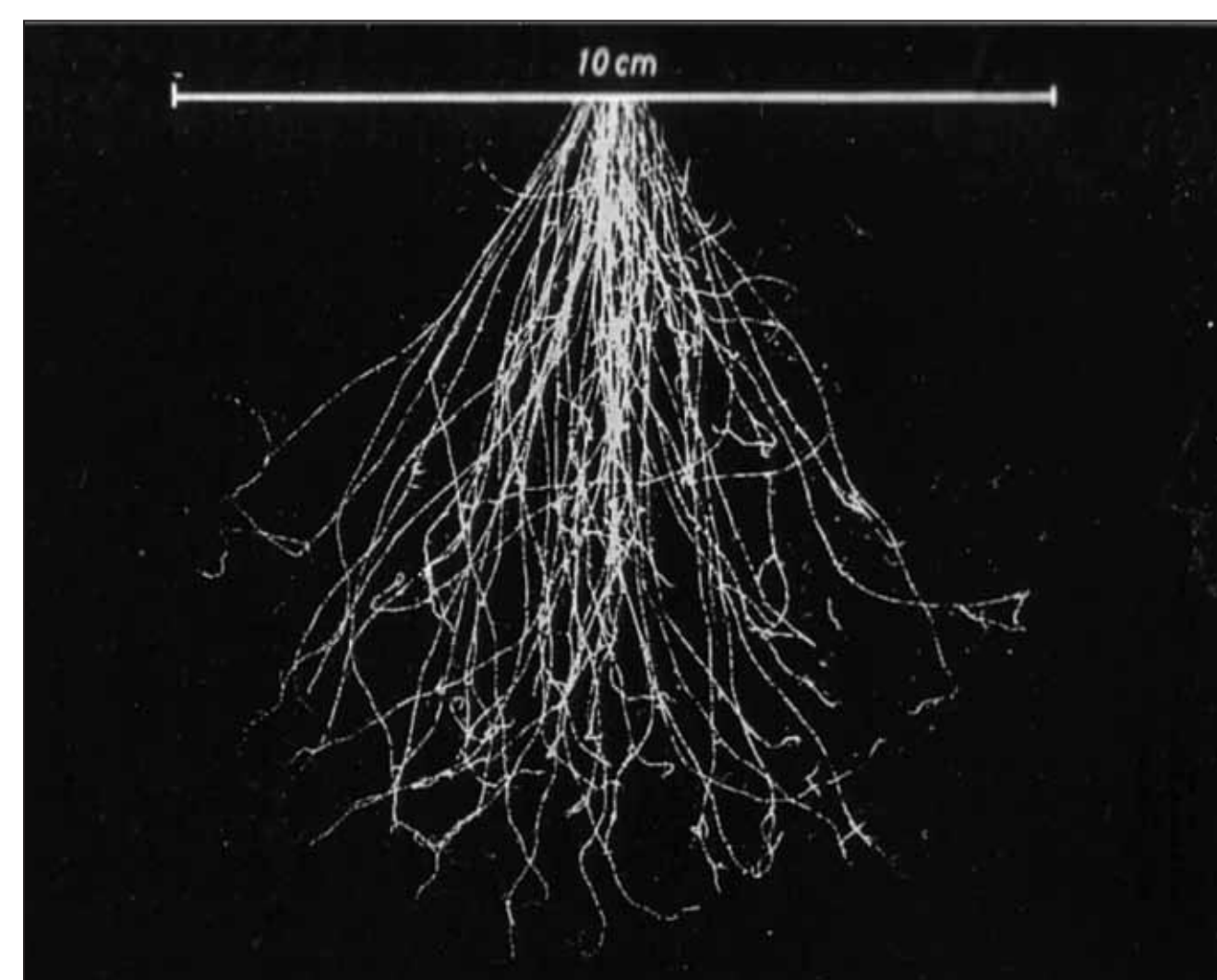
Bubble chamber picture, 7.7 MeV electrons in liquid propane.
